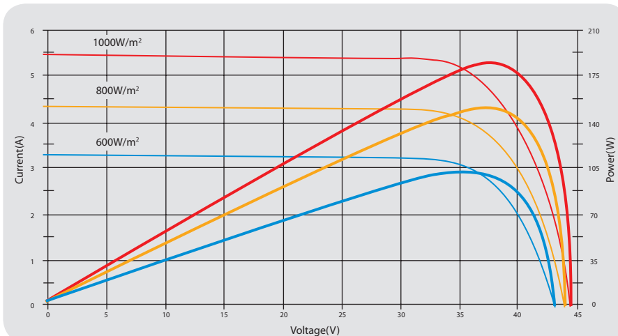
Current-Voltage & Power-Voltage Curve (185W)
